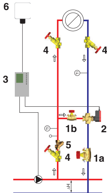
Fig. 3: Diversion circuit
