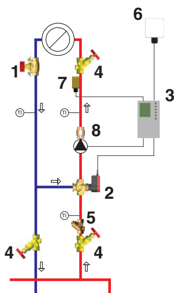
Fig. 6: Mixing circuit
