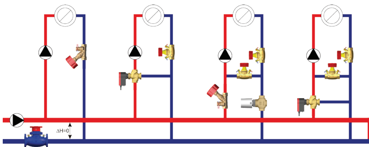
Systems with static balancing and circuit control valve, diversion circuit, injection circuit with two-port valve, dual mixing circuit.
