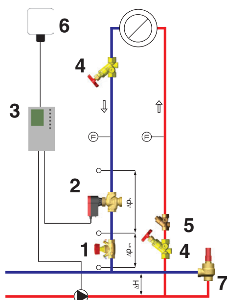
Fig. 2: throttle circuit
