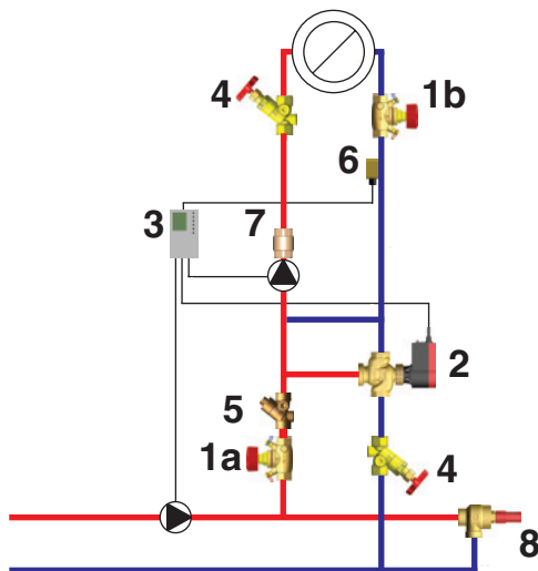
Fig. 5: Injection circuit with three-port valve
