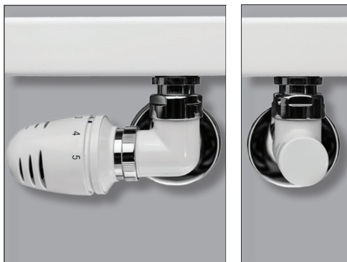
HERZ-Design Thermostatic Head MINI-GS, chrome-plated S 9200 34* Herz-TS-3-Axis Valve - "CD" - Design, chrome-plated S 7646 44* Herz-Return valve RL-Design, angle model, chrome-plated S 3745 44* Compression adapter 15 mm (2 Pcs.) S 6286 15 Pipe Cover Set, Chrome-plated S 6822 00
