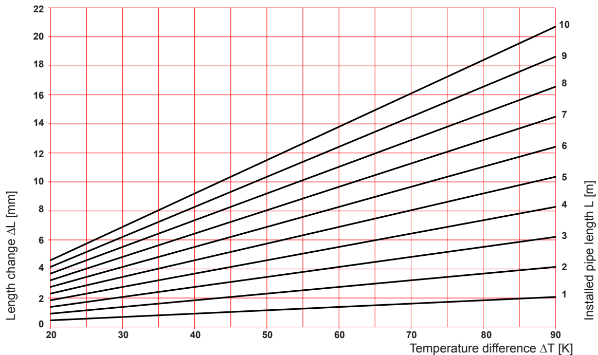
Diagram "Thermal expansion" for the aluminium multilayer pipe PipeFix
