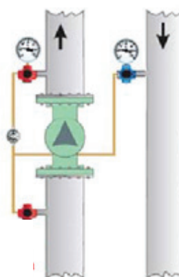
NEW 3 welds 3 possible leaks
