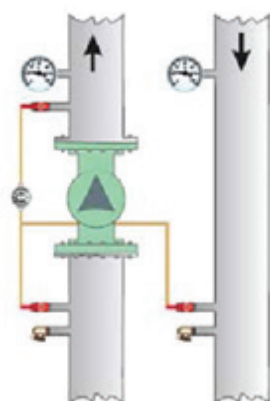
USUAL MOUNTING 7 welds 7 possible leaks
