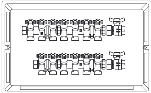
Right side connection - Straight valves
