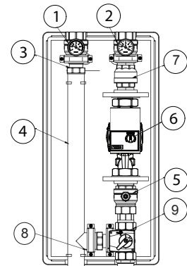
DN 40 - DN 50
