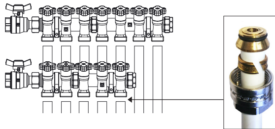
HERZ Pipefix
