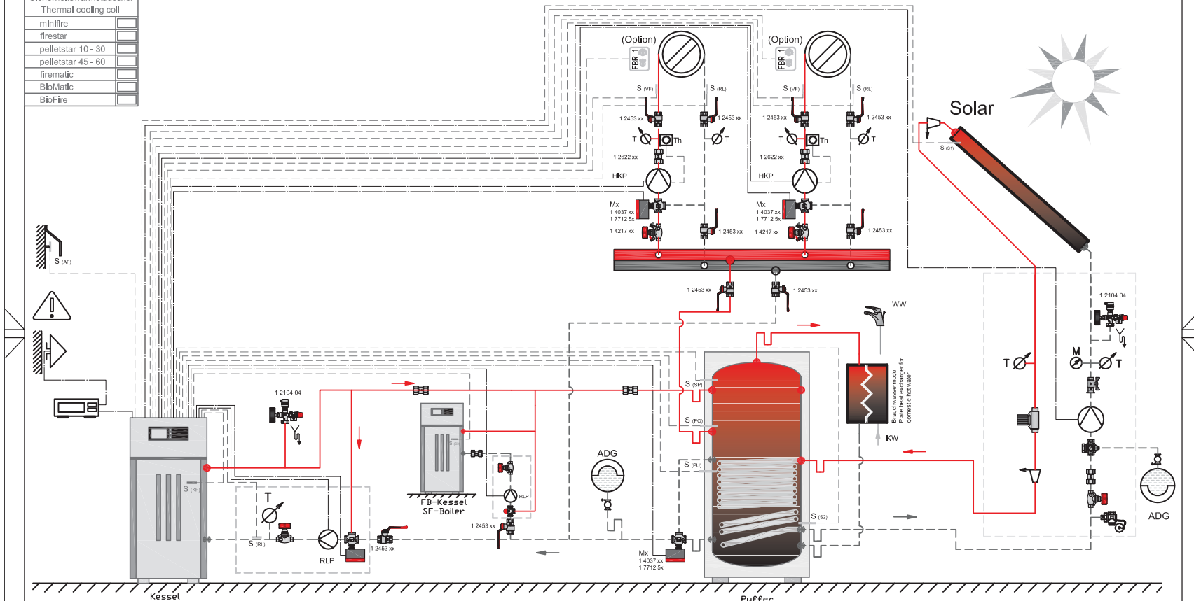
Kessel Boiler
