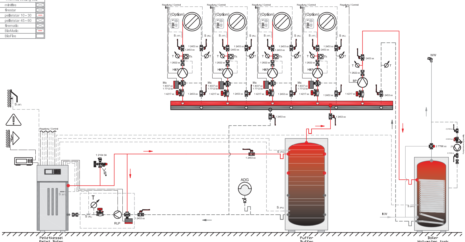
Pellekessel Pellet Boiler
