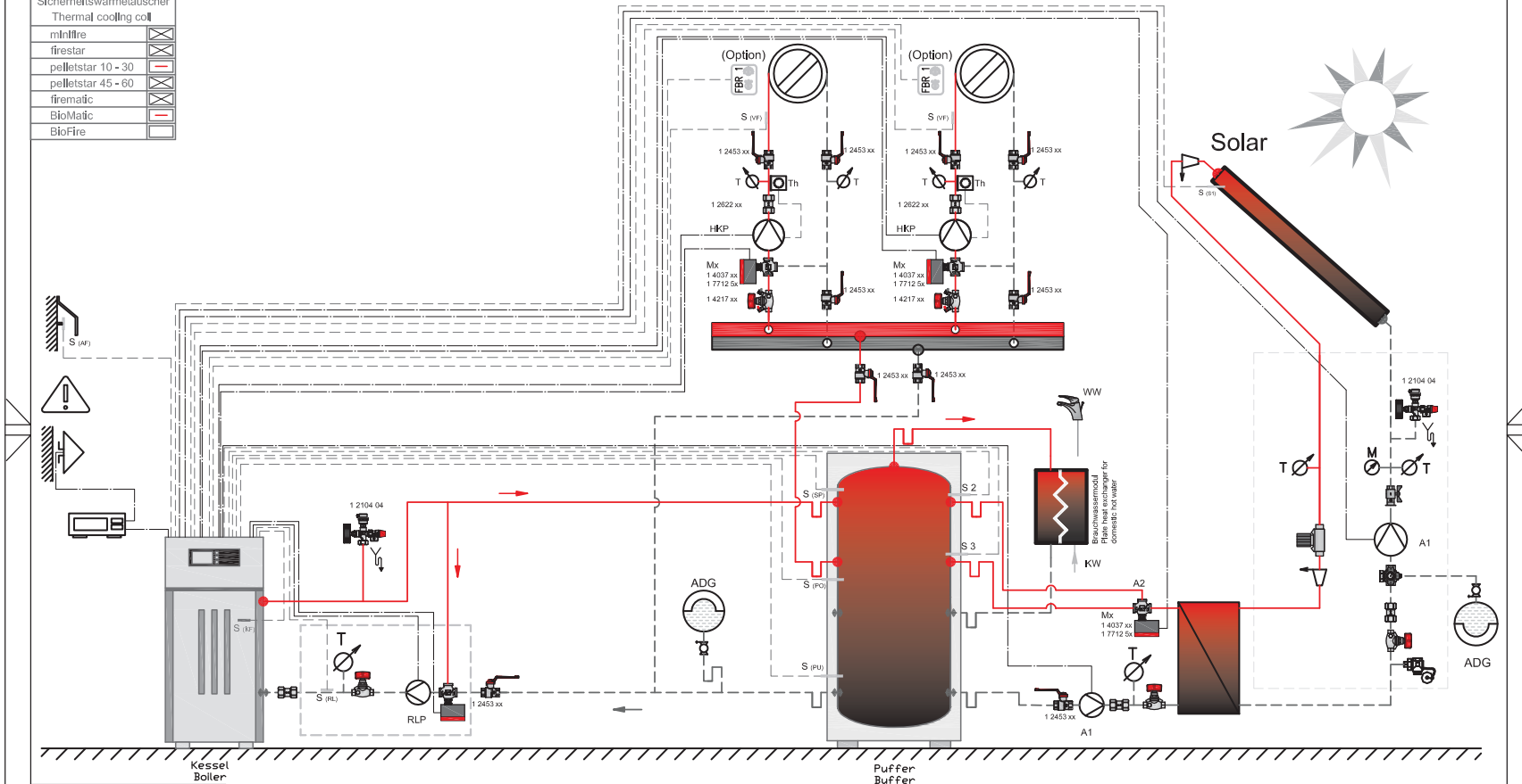
Kessel Boiler
